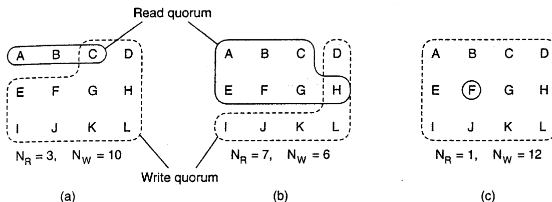
Figure 7-22. Three examples of the voting algorithm. (a) A correct choice of read and write set. (b) A choice that may lead to write-write conflicts. (c) A correct choice, known as ROW A (read one, write all).
