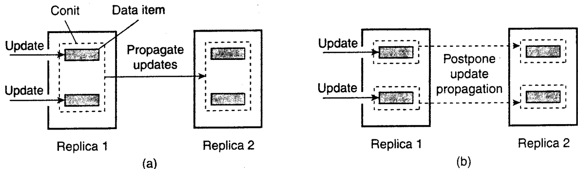
Figure 7-3. Choosing the appropriate granularity for a conit. (a) Two updates lead to update propagation. (b) No update propagation is needed (yet).
