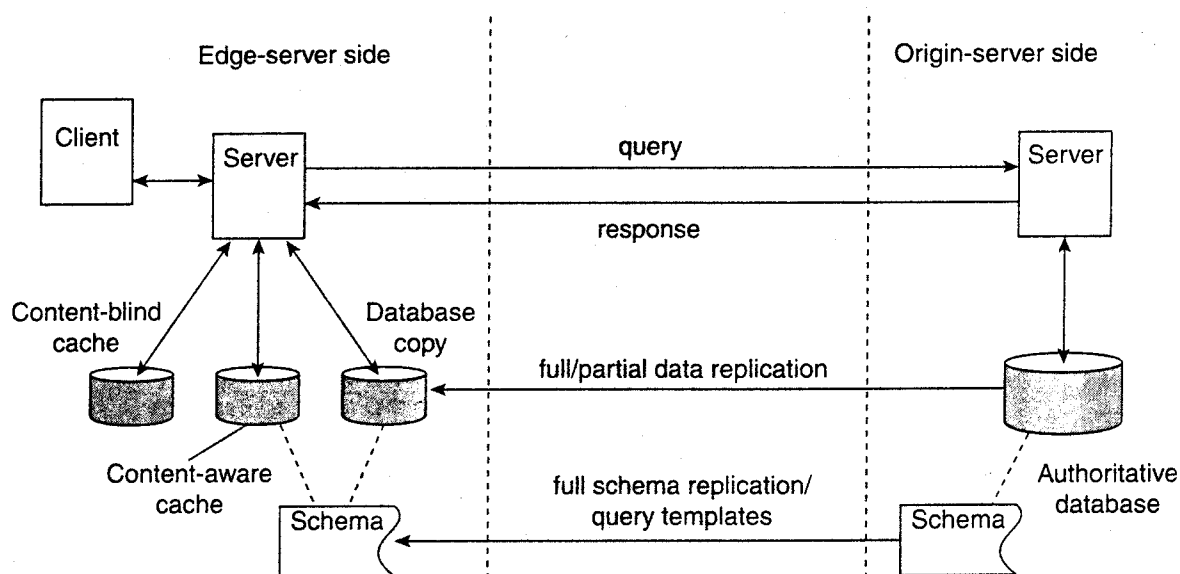
Figure 12-21. Alternatives for caching and replication with Web applications.
